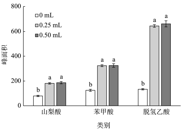
图4 盐酸浓度对峰面积的影响 Fig.4 Effects of hydrochloric acid concentration on peak area
