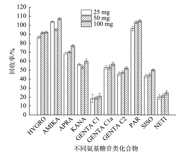
图7 不同C 18 含量对10种AGs的加标回收率统计(n=3) Fig.7 Statistical analysis of recoveries of 10 kinds of AGs with different C 18 contents (n=3)
